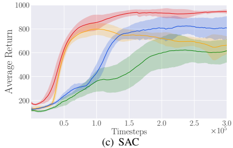
Fig. 5. Benchmarks of four RL frameworks trained with (a) PPO, (b) TD3, and (c) SAC RL algorithms. Each plot depicts the learning curves for Mono-MLP (green), Mono-EMLP (blue), Mod-MLP (orange), and Mod-EMLP (red).
